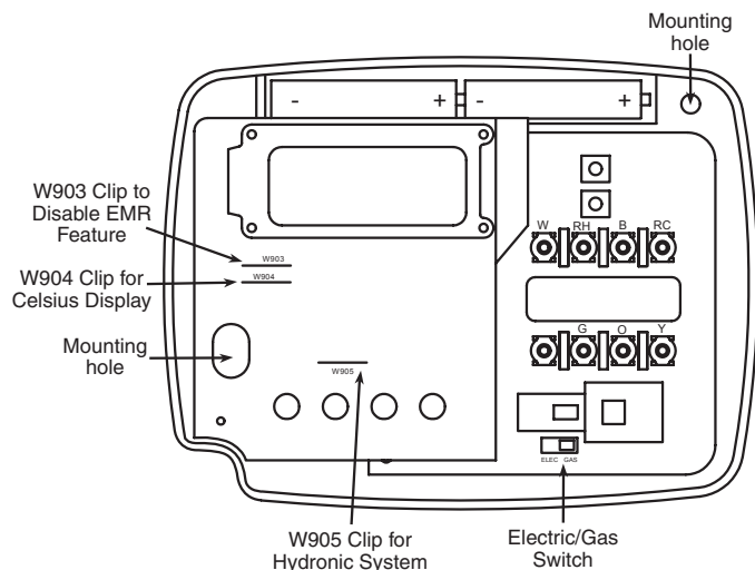
Figure 1. Thermostat base
