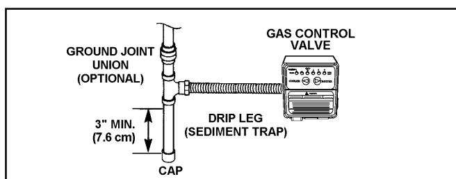
FIGURE 12. GAS PIPING WITH FLEXIBLE CONNECTOR.
