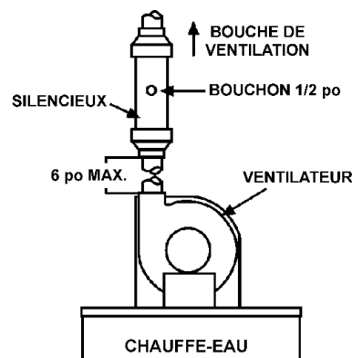
FIGURE 22 – Installation verticale type
