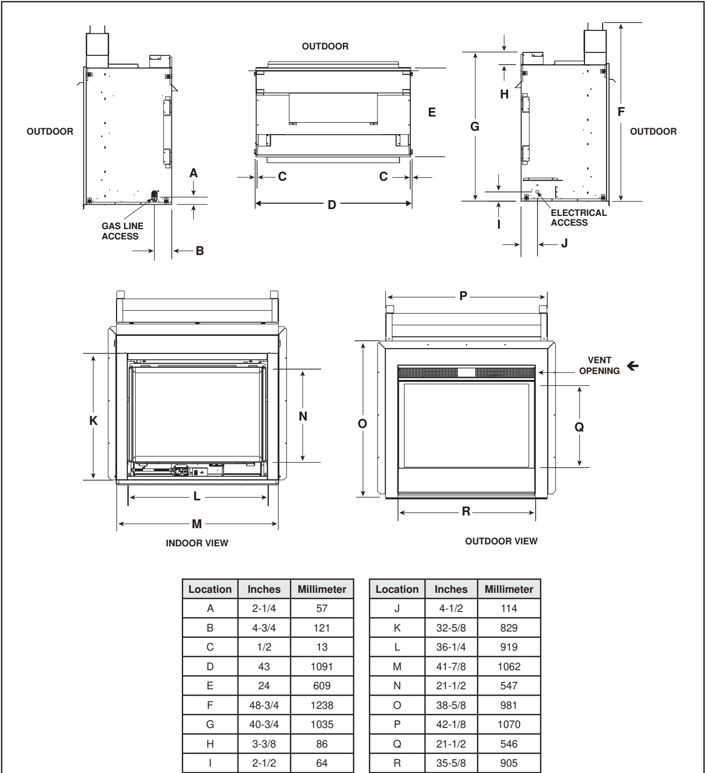
Figure 13.1 Appliance Dimensions
