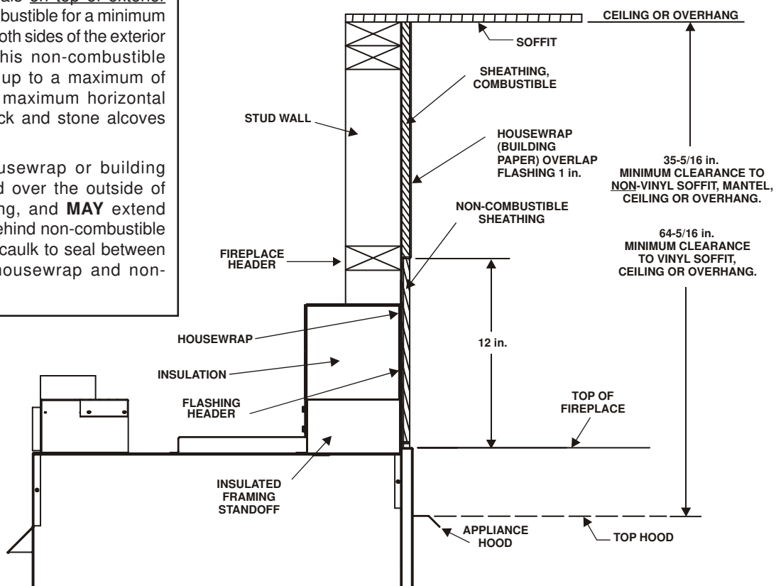
Figure 10.6 Exterior View
