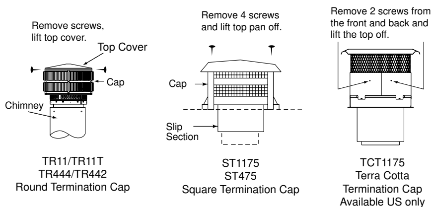
Figure 3.1 Chimney & Termination Cap Cleaning
