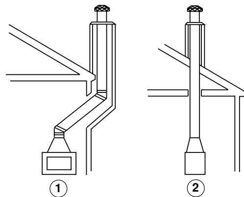
Figure 9.2 Chase Constructions
