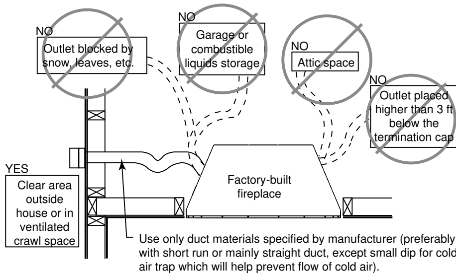
Figure 7.3 Possible Outside Air Inlet Locations
