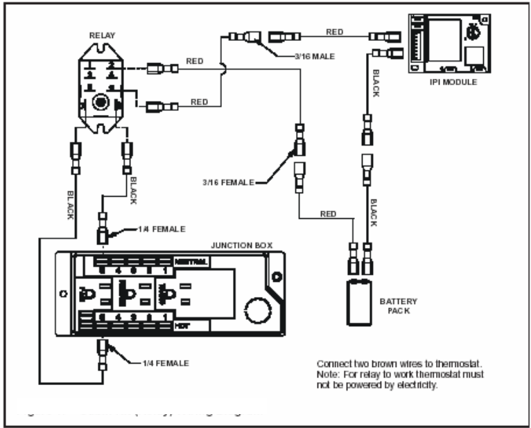
Relay Wiring
