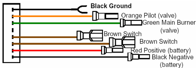
Wiring Harness
